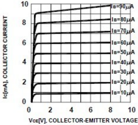
Figure 1. Static Characteristic
